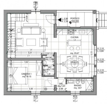
PIANO TERRA
